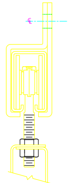
STANDARD HEAD SECTION USING HANGERS
